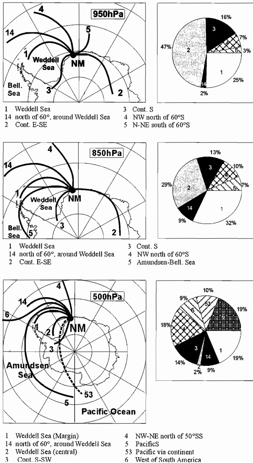
Fig. 2. Trajectory classes for three arrival levels, 950, 850 and 500 hPa, and their corresponding frequency distributions. NM: Neumayer station.
